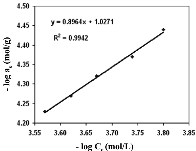
Fig. 5. Freundlich adsorption isotherm for chromate ions on Fe- \text{mPO}_4 .
