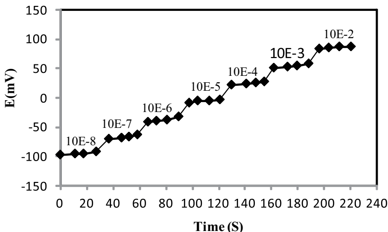
Fig. 6. Dynamic response of copper ion electrode for step changes in concentration of Cu 2+ .
