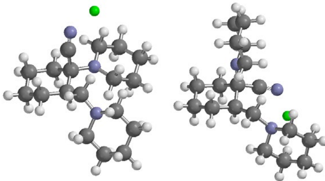
Fig. 3. Complex of ion metals (for example: Zn^{2+} ) with 1-cyano-1-piperidino-2(N-piperidino methyl)-cyclohexane ligand with axial (left) and equatorial (right) forms.
