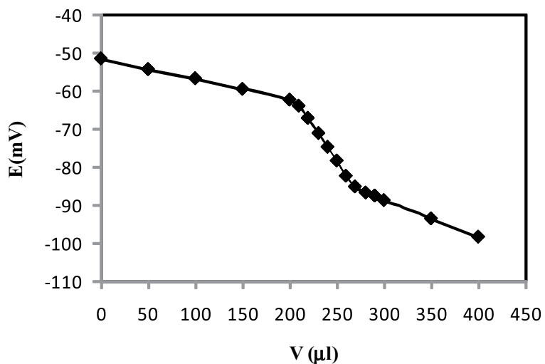
Fig. 8. Potentiometric titration curve of 1.0 \times 10^{-6} M \text{Cu}^{2+} solution with 1.0 \times 10^{-4} M EDTA using the proposed sensor as an indicator electrode.
