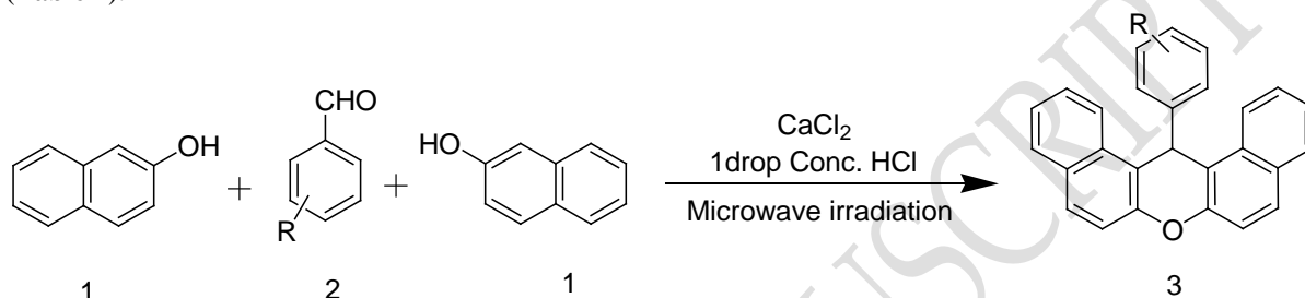
Fig. 2. Synthesis of Xanthene via one-pot condensation between 2-naphthol and benzaldehyde catalyzed by calcium chloride/Conc. HCl under microwave condition
