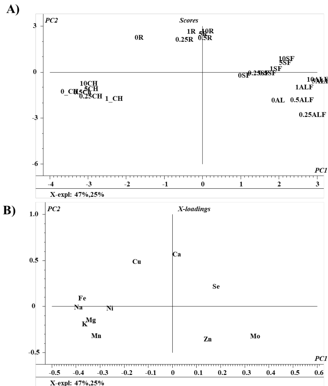
Fig 1SM. Principal components analysis (PCA) of element concentration levels found in biomass of four plants under different conditions of exposure to Se(IV): a) Two-dimensional plot of the sample scores and b) Two-dimensional plot of variable loadings in the space defined by the first two principal components.
