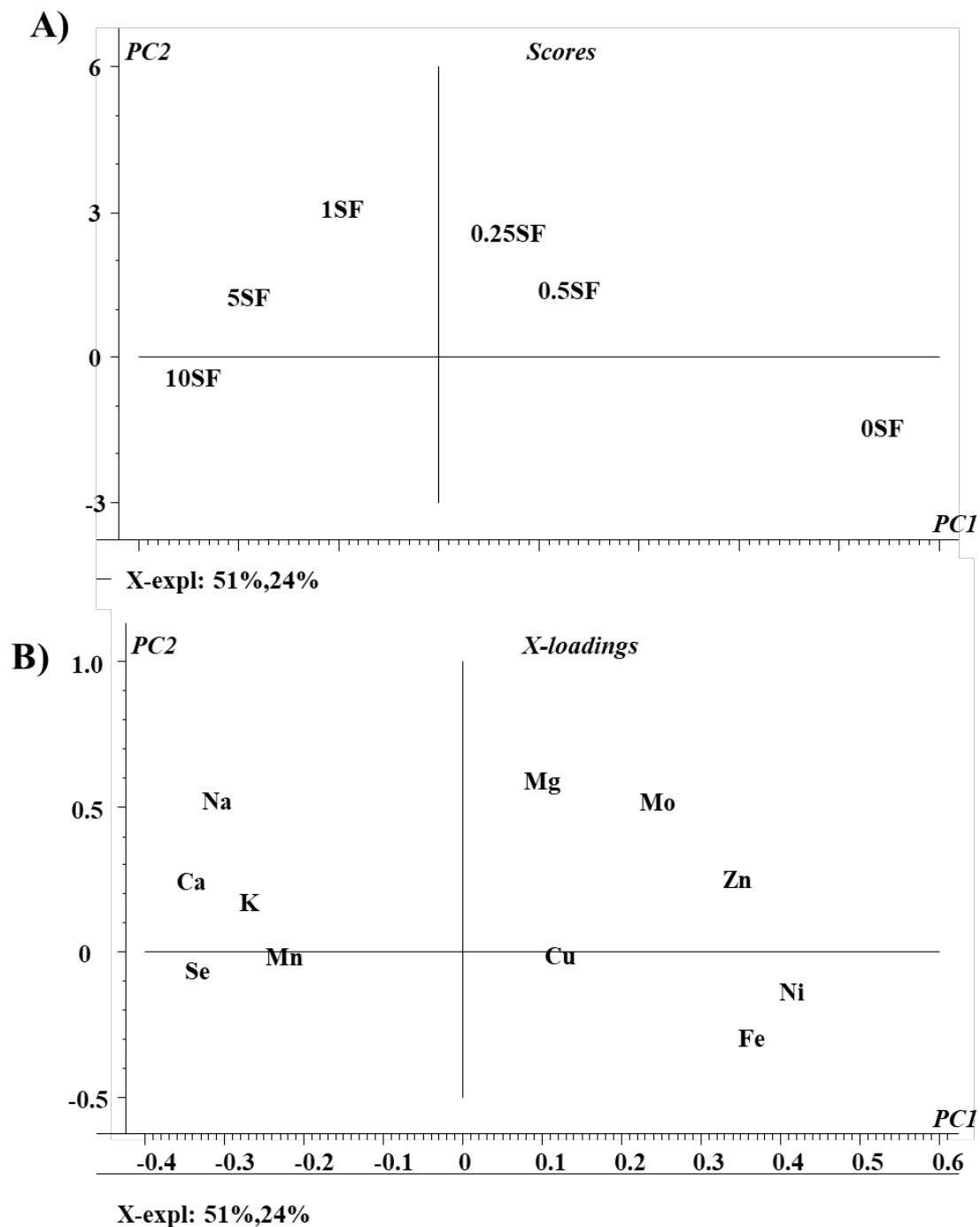
Fig 3SM. Principal components analysis (PCA) of element concentration levels found in biomass of sunflower under different conditions of exposure to Se(IV): a) Two-dimensional plot of the sample scores and b) Two-dimensional plot of variable loadings in the space defined by the first two principal components.
