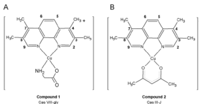
Fig. 1. Structures of the complexes studied. A: [\text{Cu}(3,4,7,8\text{-tetramethyl-1,10-phenanthroline})(\text{acetylacetonato})]^+ and B: [\text{Cu}(3,4,7,8\text{-tetramethyl-1,10-phenanthroline})(\text{glycinato})]^+ .
