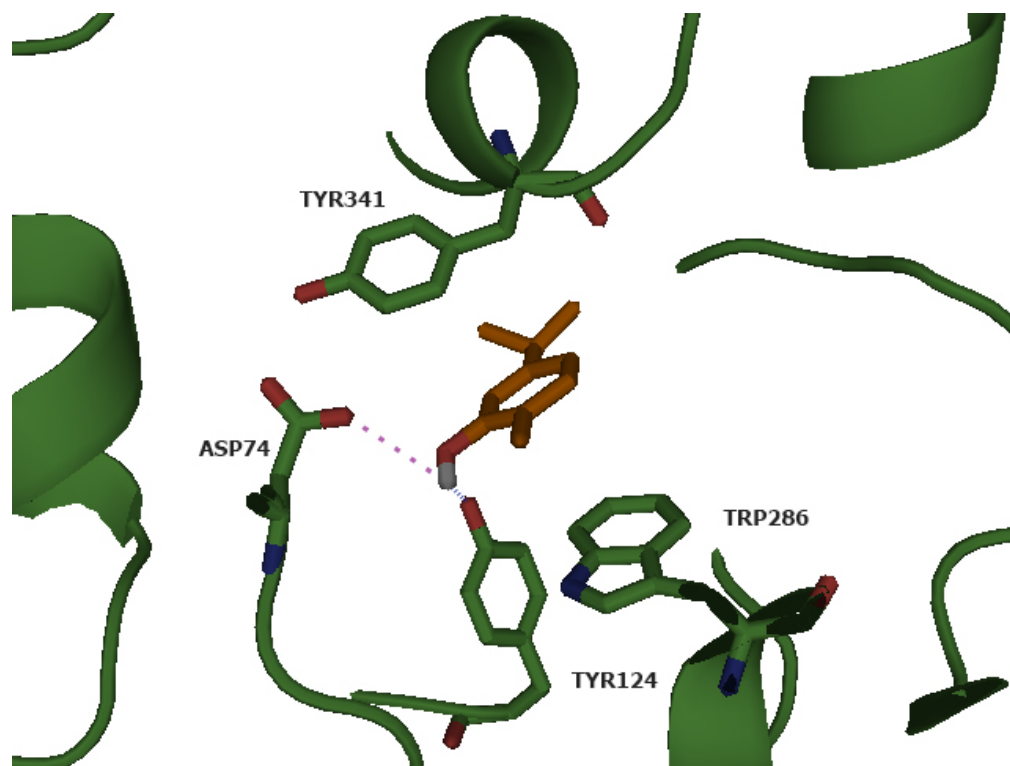
Fig. S1. Docking of Carvacrol in AChE (PDB ID: 4EY6) (Chain B). AChE is represented in green and Carvacrol in orange; O-H...O (Asp74), O-H...O (Tyr124) and C-H... \pi .
