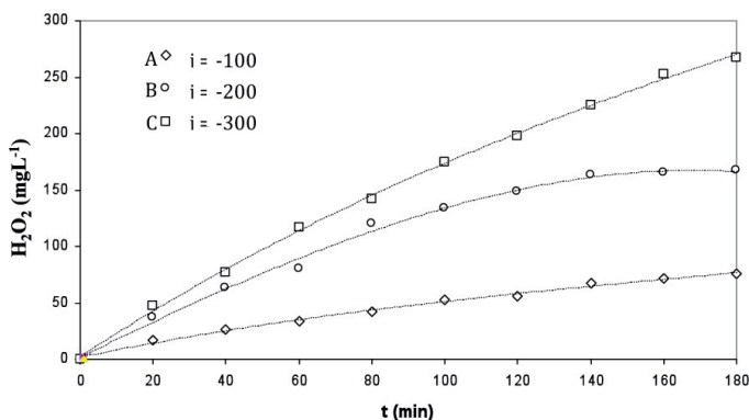
Figure 3. H 2 O 2 production in the photo-electrochemical reactor in a solution of 0.05 M Na 2 SO 4 with a flow rate of 76 L/h. The current densities were (A) 100 mA/cm 2 , (B) 200 mA/cm 2 and (C) 300 mA/cm 2 .
