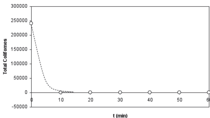
Figure 10. Abatement of total coliforms with time using the PEF system with an Fe 2+ -coated Nafion™ membrane and a TiO 2 -carbon cloth electrode.
