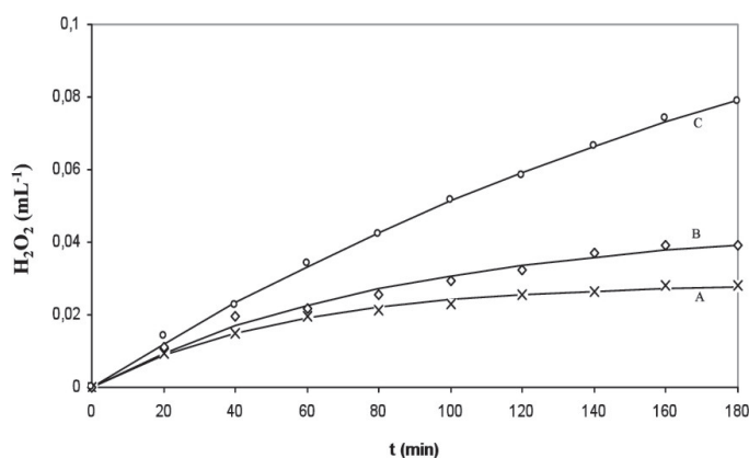
Figure 5. Simulated values obtained with a flow rate of 76 L/h and current densities of (A) 100 mA/cm 2 , (B) 200 mA/cm 2 , and (C) 300 mA/cm 2 .
