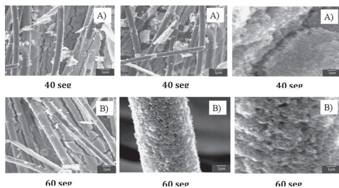
Figure 9. SEM images of carbon cloth fibers coated with TiO 2 . (a) Deposition time of 40 s, T = 450 °C for 30 min. (b) Deposition time of 60 s, T = 450 °C for 30 min.
