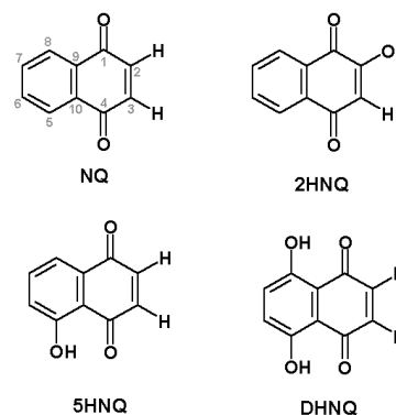
Figure 2. Structures for studied quinonoid compounds: NQ: 1,4-naphthoquinone; 2HNQ: 2-hydroxy-1,4-naphthoquinone; 5HNQ: 5-hydroxy-1,4-naphthoquinone, DHNQ, 5, 8-dihydroxy-1,4-naphthoquinone.
