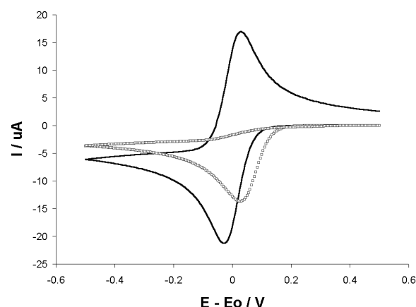
Figure 5. Simulated cyclic voltammograms for single electron transfer process (solid line), and ECEC self-protonation process (dotted line). Simulation conditions are: C_0 : 1 \times 10^{-3} mol L ^{-1} , working electrode area: 0.025 cm ^2 , D_0 : 1.9 \times 10^{-5} cm ^2 s ^{-1} ; v : 1000 mV s ^{-1} . All standard rate of electron transfer constants were set to 0.05 cm s ^{-1} . Self-protonation reactions (equations 4 and 6) were simulated using K_{eq} = 10000 and k_f = 1000000 .
