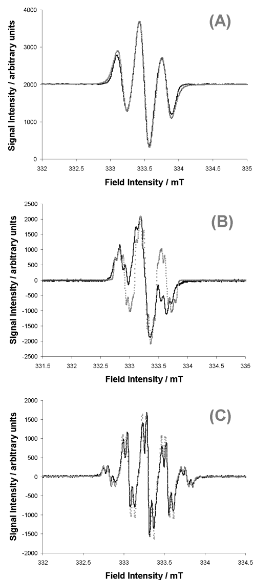
Figure 8. ESR spectra obtained for different quinoid compounds in the potential region for semiquinone formation. A: 5 \times 10^{-4} mol L -1 1,4-naphthoquinone NQ semiquinone (Applied potential: -1.24 V vs Fc +/0 /Fc); B: 1.1 \times 10^{-3} mol L -1 5-hydroxy-1,4-naphthoquinone 5HNQ semiquinone (Applied potential: -1.08 V vs Fc +/0 /Fc); C: 1.1 \times 10^{-3} mol L -1 5, 8-dihydroxy-1,4-naphthoquinone DHNQ semiquinone (Applied potential: -1.02 V vs Fc +/0 /Fc). Solid line represents experimental spectrum. Dotted line depicts simulated one.
