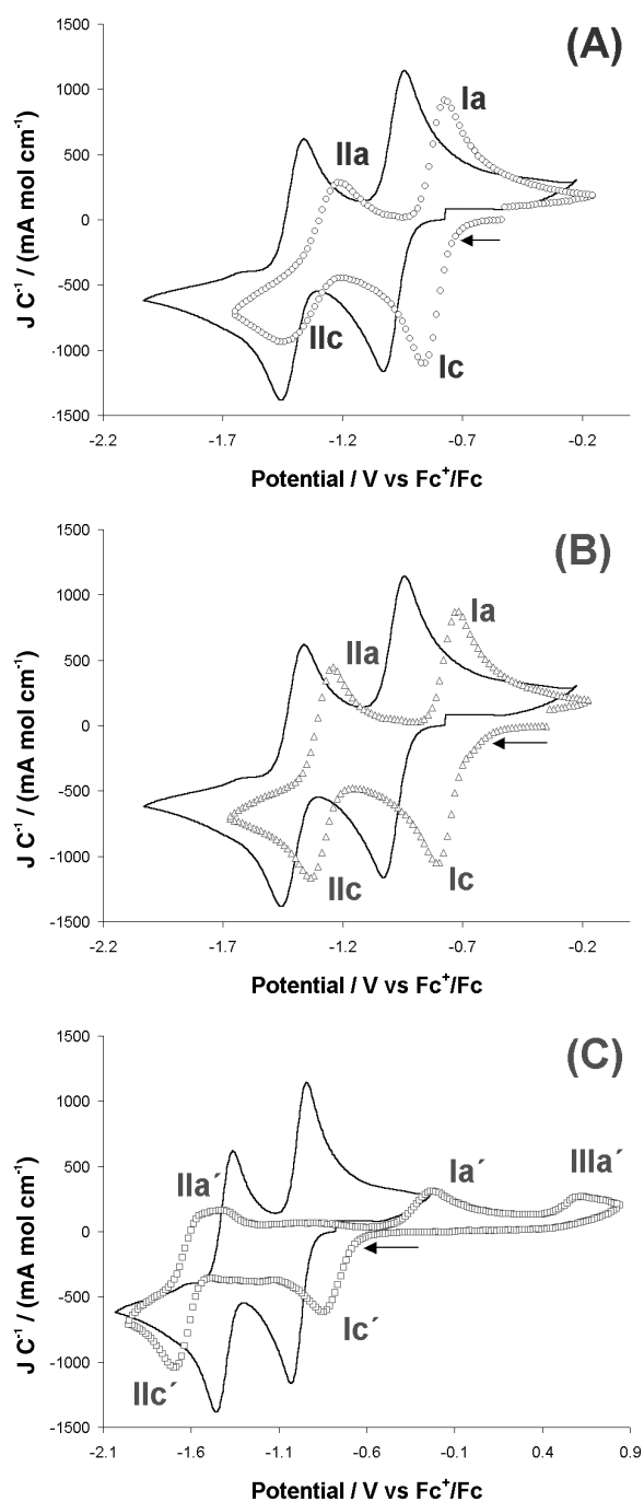
Figure 3. Typical cyclic voltammograms of (A, \circ ) 6.3 \times 10^{-3} mol L ^{-1} 5-hydroxy-1,4-naphthoquinone 5HNQ; (B, \triangle ) 5.7 \times 10^{-3} mol L ^{-1} , 5,8-dihydroxy-1,4-naphthoquinone DHNQ and (C, \square ) 3.9 \times 10^{-3} mol L ^{-1} 2-hydroxy-1,4-naphthoquinone 2HNQ in 0.1 mol L ^{-1} Et _4 NBF _4 /CH _3 CN. Platinum surface: 0.025 cm ^2 v: 1000 mVs ^{-1} . 5.1 \times 10^{-3} mol L ^{-1} ; 1,4-naphthoquinone, is used as comparison with each compound as a solid line inner voltammogram. Both cathodic and anodic peaks are indicated.
