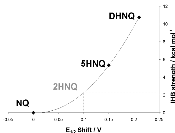
Figure 4. Shift in the half-wave potential vs. IHB strength relationship for 1,4-naphthoquinone NQ, 5-hydroxy-1,4-naphthoquinone 5HNQ and 5, 8-dihydroxy-1,4-naphthoquinone DHNQ (for which sum of IHB strength is plotted in the graph). The estimated shift value for 2-hydroxy-1,4-naphthoquinone is obtained by interpolation in this curve.
