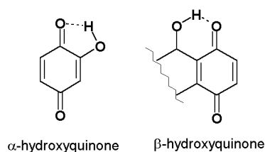
Figure 1. Main structures in \alpha and \beta -hydroxyquinones. Intramolecular hydrogen bond interactions are depicted by the dashed line.
