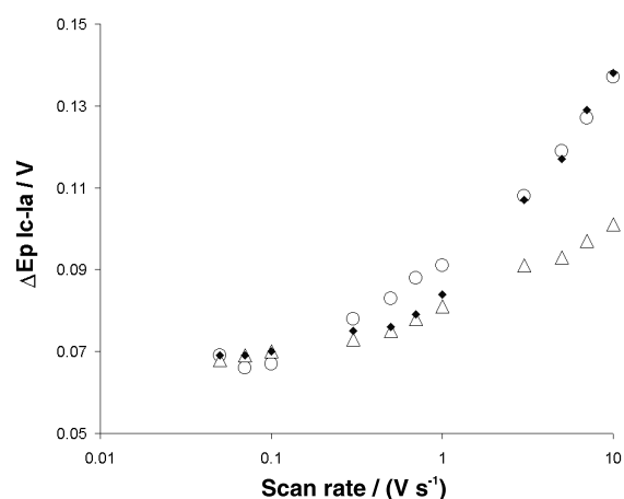
Figure 6. Peak potential difference Ic-Ia, for 1, 4-naphthoquinone (NQ, \blacklozenge ); 5-hydroxy-1,4-naphthoquinone (5HNQ, \circ ) and 5, 8-dihydroxy-1,4-naphthoquinone (DHNQ, \triangle ), as a function of the scan rate. Hermano, dá pra usar (V s -1 ) ?
