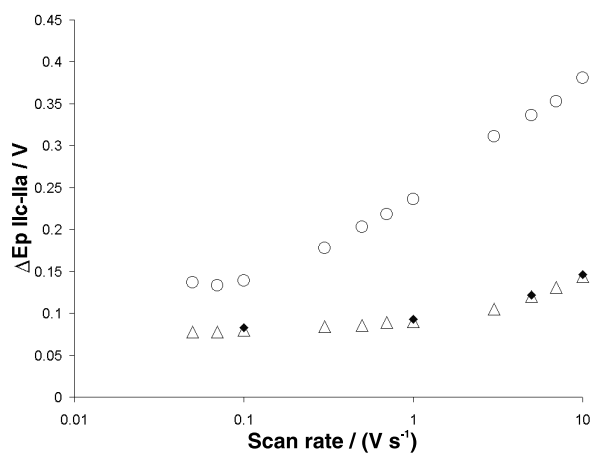
Figure 7. Peak potential difference IIC-IIa, for 1, 4-naphthoquinone (NQ, \blacklozenge ); 5-hydroxy-1,4-naphthoquinone (5HNQ, \circ ) and 5, 8-dihydroxy-1,4-naphthoquinone (DHNQ, \triangle ), as a function of the scan rate.
