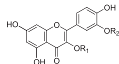
47a R 1 = H R 2 = H 47b R 1 = Gluc R 2 = H 47c R 1 = Gluc 6 -OAc R 2 = H 47d R 1 = Gluc R 2 = Me 47e R 1 = Gluc 6 -OAc R 2 = Me 47f R 1 = Gal R 2 = Me 47g R 1 = Gluc 3 -Rhamn R 2 = H 47h R 1 = Rhamn R 2 = H 47i R 1 = Gal R 2 = H 47j R 1 = Gal 2 -OAc R 2 = H
