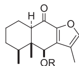
128a 128b 128c 128d 128e 128f R A MeBut Ang C MeBut /Val Δ 1,10 Δ 1,10 Δ 1,10
