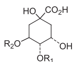
135a R 1 = R 2 = caffeoyl 135b R 1 = H R 2 = caffeoyl
