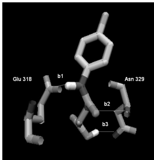
Fig. 6. Interactions and distances between the compound 1b and the Asn329 and Glu318.
